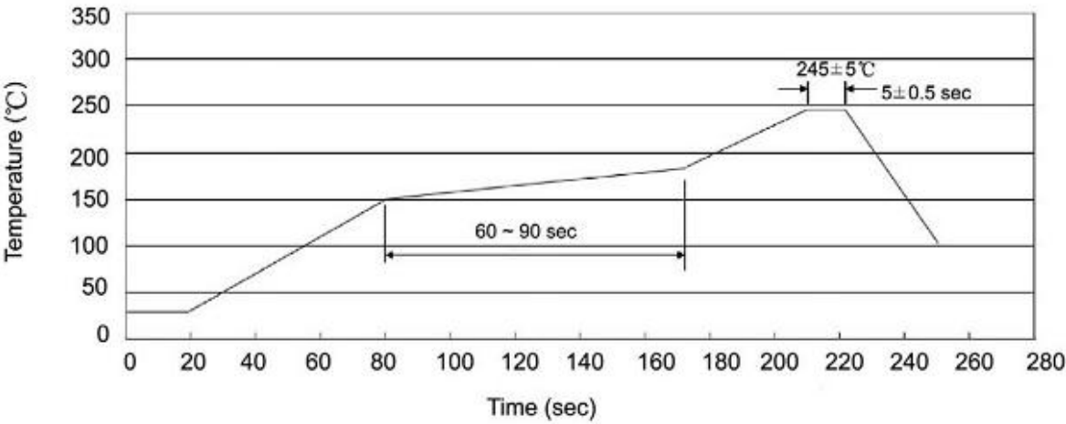
Temperature Profile for IR Reflow Soldering(Pb-Free)
