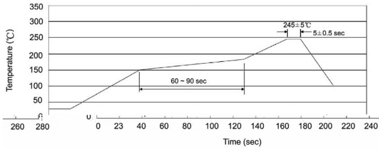
( ) / Temperature Profile for Dip Soldering(Pb-Free)
